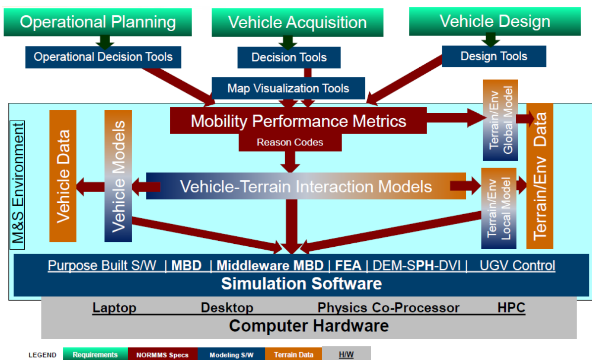
Figure 7-2: Next-Generation NRMM Schematic and NORMMS Requirements Flow.
